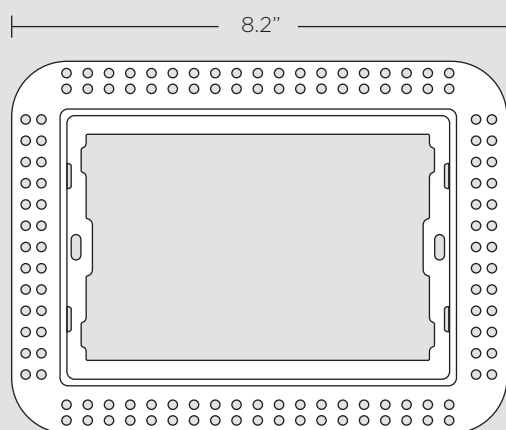
BRACKET FRONT VIEW
